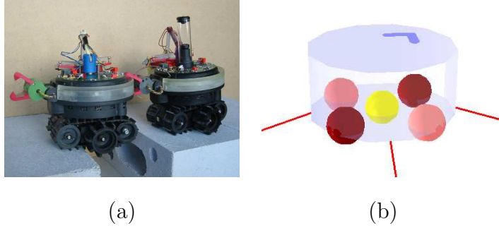
Figure 1. (a) Two s-bots physically connected showing how is it possible to pass over a gap exploiting the cooperation. The s-bot is provided with a traction system comprising wheels and tracks, a rotating turret holding the rigid and the flexible grippers, and many sensors. (b) The simulated s-bot model. The turret is transparent to show the chassis (centre sphere), the motorised wheels (lighter spherical wheels) and the passive wheels (darker spherical wheels). The position of the gripper is shown with an arrow painted on the s-bot 's body. Ground sensors are displayed as lines exiting from the s-bot .
