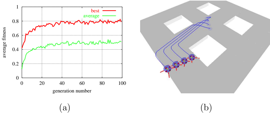
Figure 2. Hole avoidance results: (a) Average fitness over 10 replications of the experiment. (b) Trajectories displayed by a swarm-bot performing a hole avoidance task.
