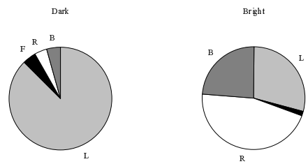
Figure 12. Percentage of time each of the four input units is the most active one during one epoch without learning (i.e., using the weight values inherited at birth) in both the dark and bright environment. The measures are carried out on an individual evolved to learn during lifetime. (F=front sensor (black); B=back sensor (dark-gray); L=left sensor (light-gray); R=right sensor (white)).
