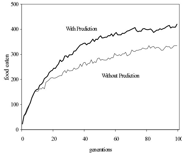
Figure 4. Average of food tokens eaten by populations of animats throughout generations for experiments with and without learning. Each curve is the average result of 10 replications. The difference between the two curves is statistically significant from generation 25 (see Nolfi, Elman, and Parisi, 1994).
