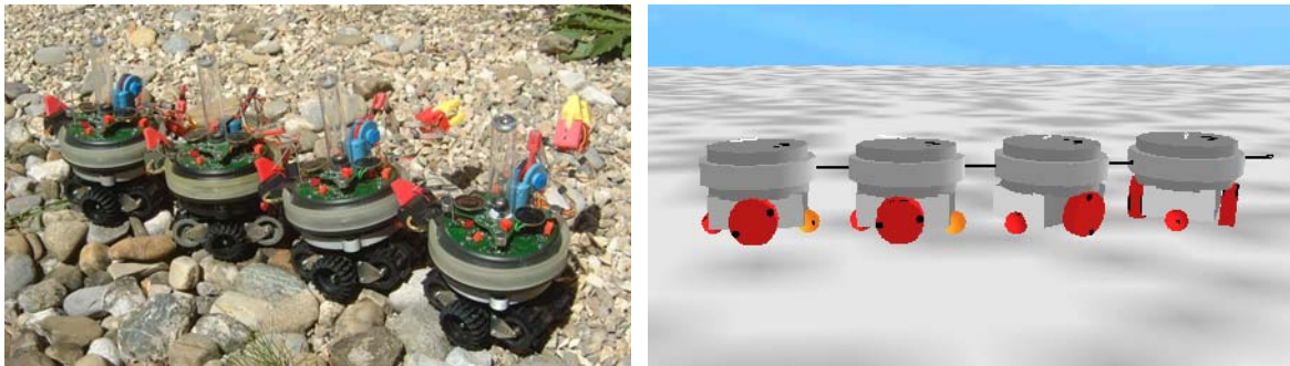
Figure 5. Left: Four robots assembled into a linear structure. Right: A simplified simulation of the robots described in the left part of the figure based on Vortex™ libraries.
