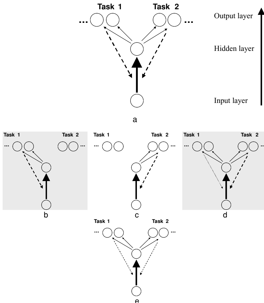
Figure 7. Neural interference between the What task and the Where task in a nonmodular network architecture. The solid lines represent connection weights, while the dotted lines represent error messages (the thicker is the dotted line, the bigger is the error message). An early stage of simultaneous learning of the two task is shown in (a), while four succeeding stages of sequential learning are shown in (b)–(e) (for more details, see the text).
